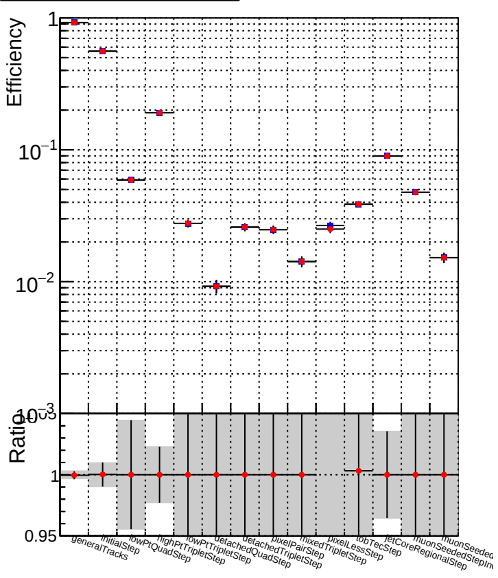
DQM_V0001_R000000001_Global_mkFitbase_RECO DQM_V0001_R000000001_Global_mkFit-cand_RECO
