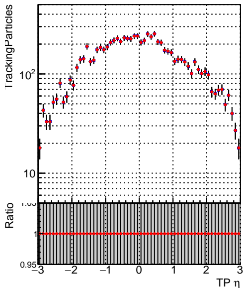
— DQM_V0001_R000000001_Global_mkFitbase_RECO — DQM_V0001_R000000001_Global_mkFit-cand_RECO
