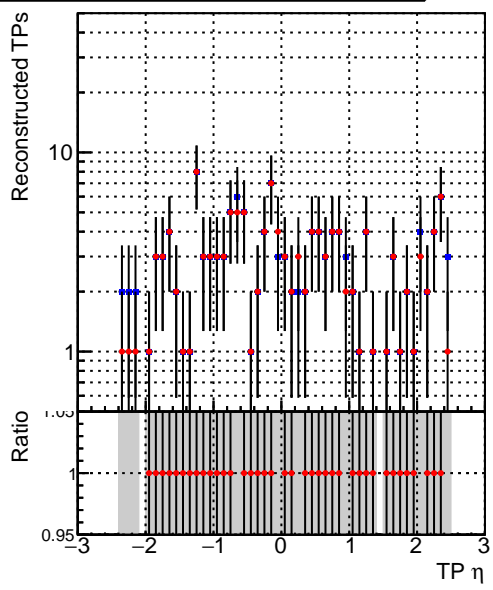
N of simulated tracks vs \eta Legend: - DQM_V0001_R000000001_Global_mkFitbase_RECO (blue diamonds) - DQM_V0001_R000000001_Global_mkFit-cand_RECO (red diamonds)
