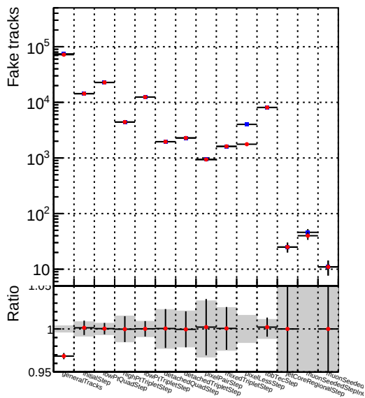
Number —●— DQM_V0001_R000000001_Global_mkFit-cand_RECO
