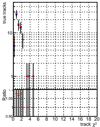
N of reco track vs. \chi^2 —●— DQM_V0001_R000000001_Global_mkFitbase_RECO —●— DQM_V0001_R000000001_Global_mkFit-cand_RECO
