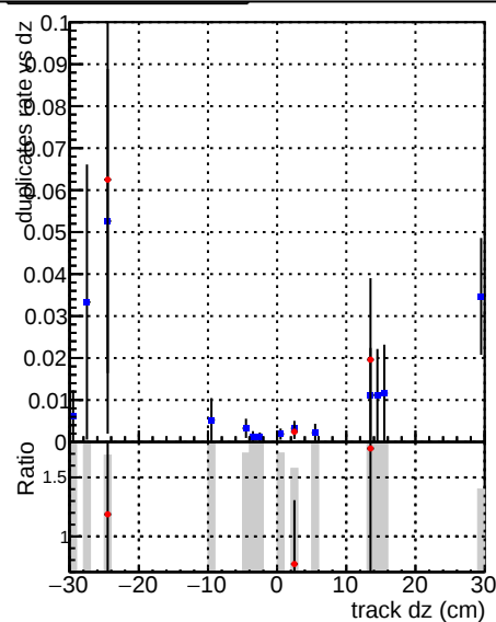
—●— DQM_V0001_R0000000001 Global mkFitbase RECO —●— DQM_V0001_R0000000001 Global mkFit-cand RECO
