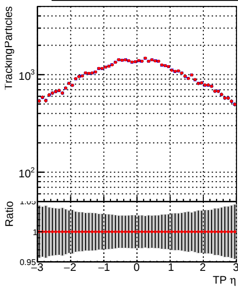
Legend: DQM_V0001_R000000001_Global_mkFitbase_RECO (blue line), DQM_V0001_R000000001_Global_mkFit-cand_RECO (red line)
