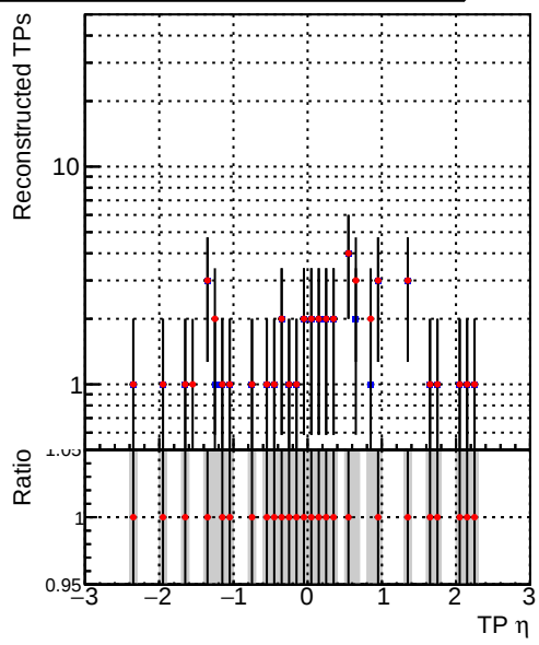
Legend: DQM_V0001_R000000001_Global_mkFitbase_RECO (blue line), DQM_V0001_R000000001_Global_mkFit-cand_RECO (red line)
