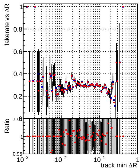
—●— DQM_V0001_R000000001_Global_mkFitbase_RECO —●— DQM_V0001_R000000001_Global_mkFit-cand_RECO
