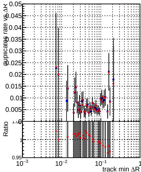
—●— DQM_V0001_R000000001_Global_mkFitbase_RECO —●— DQM_V0001_R000000001_Global_mkFit-cand_RECO
