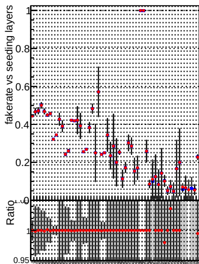
Fake rate vs. Legend DQM V0001_R000000001 Global mkFitbase RECO Blue circle Global mkFitbase RECO Red circle Global mkFitbase RECO
