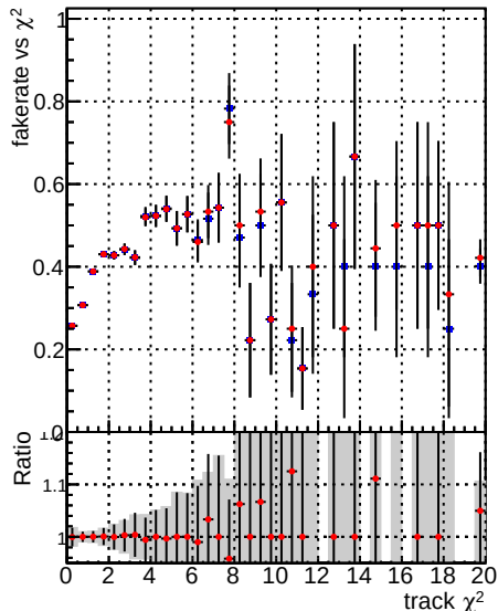
Fake rate vs. —●— DQM V0001_R000000001 Global mkFitbase RECO —●— DQM V0001_R000000001 Global mkFit-cand RECO
