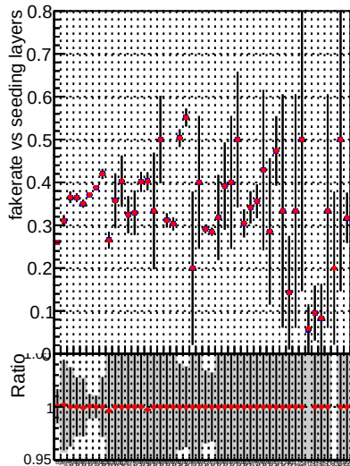
Fake rate vs. —●— DQM V0001_R000000001 Global mkFitbase RECO —●— DQM V0001_R000000001 Global mkFit-cand RECO
