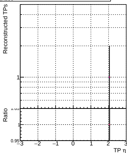
N of sim Color DOM V0001 R0000000001 Global mkFitOPY RECO Red DOM V0001 R0000000001 Global mkFitOPY RECO Black DOM V0001 R0000000001 Global mkFitOPZ RECO Orange DOM V0001 R0000000001 Global mkFitOPT RECO
