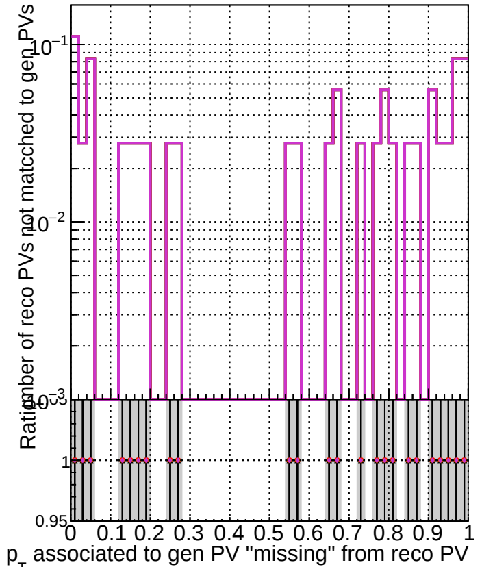
RecoPVAssoc2GenPVnotmatched_missing
