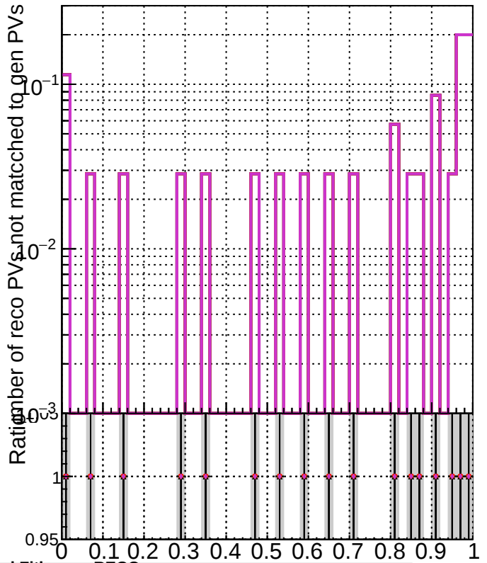
RecoPVAssoc2GenPVNotMatched_Purity
