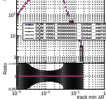
N of reconstructed tracks vs dR(track,jet)
