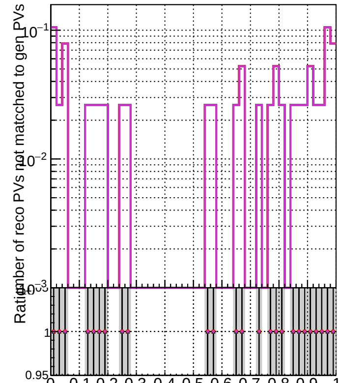
RecoPVAssoc2GenPVNotMatched_missing
