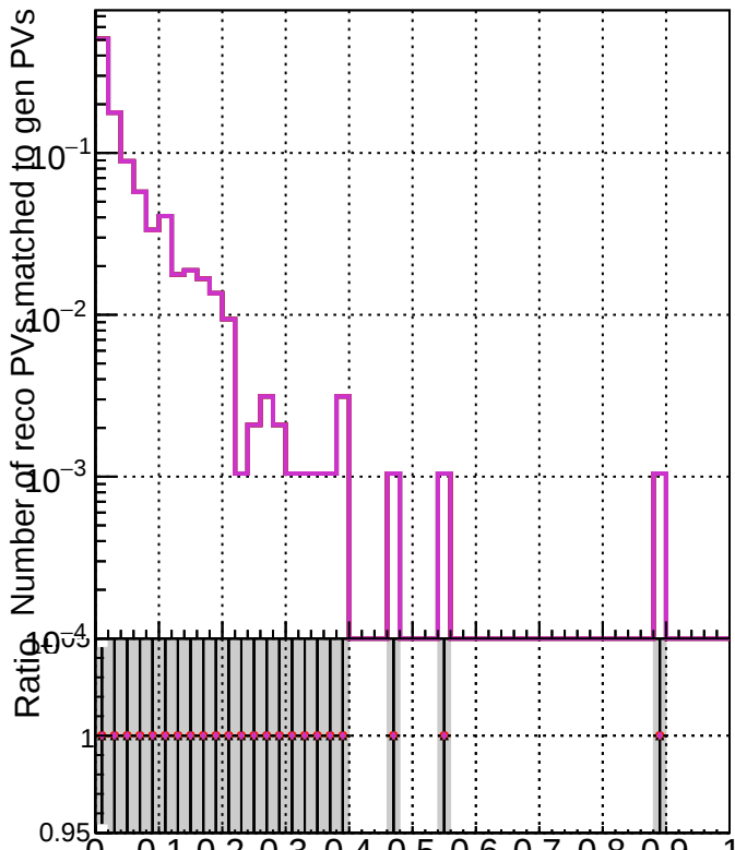
RecoPVAssoc2GenPVMatched_missing
