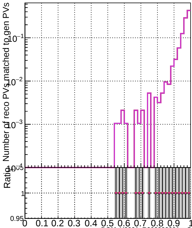
RecoPVAssoc2GenPVMatched_Purity
