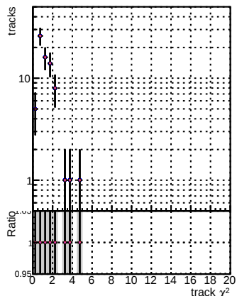
N of reco track vs. \chi^2 for BOM V0001, B0000000001, Global mxFitbase, RECO, Global mxFitbase, RECO, Global mxFitbase, RECO
