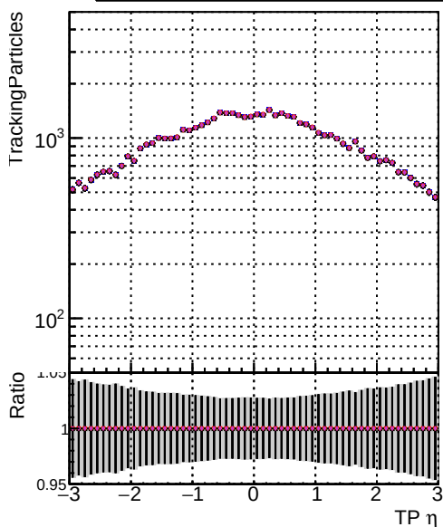
N of sin DOM V0001 R0000000001 Global mkFitOPY RECO DOM V0001 R0000000001 Global mkFitOPZ RECO DOM V0001 R0000000001 Global mkFitOPT RECO
