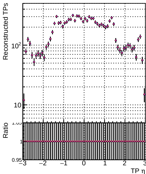
N of sim Algorithm DOM V0001 R0000000001 Global mkFitOPY RECO DOM V0001 R0000000001 Global mkFitOPY RECO DOM V0001 R0000000001 Global mkFitOPZ RECO DOM V0001 R0000000001 Global mkFitOPT RECO
