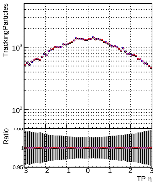
N of sim Algorithm DOM V0001 R0000000001 Global mkFitOPY RECO DOM V0001 R0000000001 Global mkFitOPY RECO DOM V0001 R0000000001 Global mkFitOPZ RECO DOM V0001 R0000000001 Global mkFitOPT RECO
