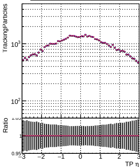
N of sim DOM V0001 R0000000001 Global mkFitOPY RECO DOM V0001 R0000000001 Global mkFitOPZ RECO DOM V0001 R0000000001 Global mkFitOPT RECO
