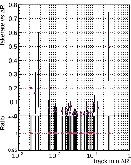
Fake rate vs \Delta R(\text{track}, \text{jet}) DQM V00001 R000000000001 Global mkFitbase BEGO Global mkFitbase BEGO Global mkFitbase BEGO Global mkFitbase BEGO
