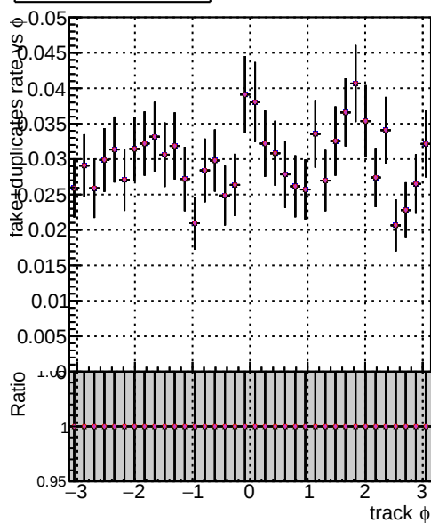
fake+duplicates vs \emptyset
