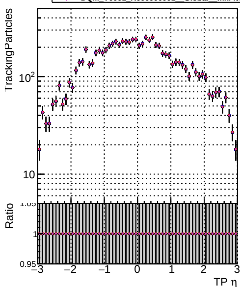
N of sim DOM V0001 R00000000001 Global mkc Filebase RECO 1 DOM V0001 R00000000001 Global mkc Filebase RECO 2 DOM V0001 R00000000001 Global mkc Filebase RECO 3 DOM V0001 R00000000001 Global mkc Filebase RECO 4 DOM V0001 R00000000001 Global mkc Filebase RECO 5 DOM V0001 R00000000001 Global mkc Filebase RECO 6 DOM V0001 R00000000001 Global mkc Filebase RECO 7 DOM V0001 R00000000001 Global mkc Filebase RECO 8 DOM V0001 R00000000001 Global mkc Filebase RECO 9 DOM V0001 R00000000001 Global mkc Filebase RECO 10 DOM V0001 R00000000001 Global mkc Filebase RECO
