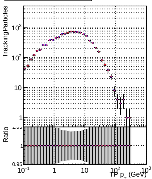
N of sim DOM V0001 R00000000001 Global mkc Filebase RECO 1 DOM V0001 R00000000001 Global mkc Filebase RECO 2 DOM V0001 R00000000001 Global mkc Filebase RECO 3 DOM V0001 R00000000001 Global mkc Filebase RECO 4 DOM V0001 R00000000001 Global mkc Filebase RECO 5 DOM V0001 R00000000001 Global mkc Filebase RECO 6 DOM V0001 R00000000001 Global mkc Filebase RECO 7 DOM V0001 R00000000001 Global mkc Filebase RECO 8 DOM V0001 R00000000001 Global mkc Filebase RECO 9 DOM V0001 R00000000001 Global mkc Filebase RECO 10 DOM V0001 R00000000001 Global mkc Filebase RECO
