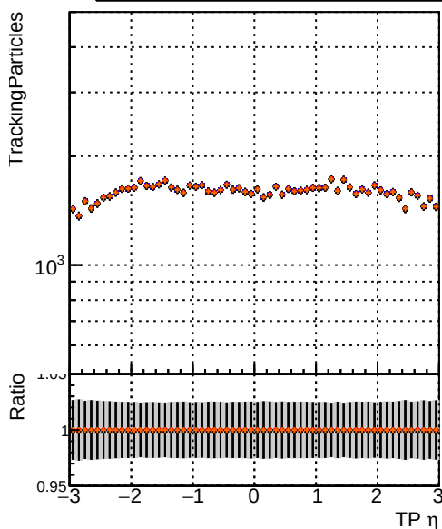
N of sim Model Fit Model Fit 1 DQM V0001 R0000000001 Global mkFitNDOF RECO 2 DQM V0001 R0000000001 Global mkFitNDOF RECO 3 DQM V0001 R0000000001 Global mkFitNDOF2 RECO
