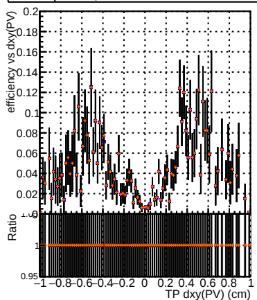
Efficienc — DQM_V0001_R0000000001_Global_mkFitNDOF_RECO — DQM_V0001_R0000000001_Global_mkFitNDOF2_RECO
