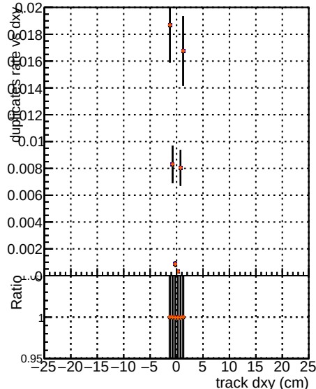
al=mkFitNBOF2-RECO al=mkFitNBOF2-RECC
