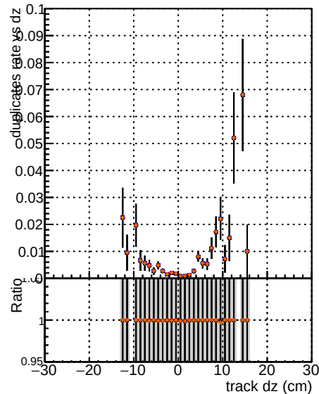
al=mkFitNBOF2-RECO al=mkFitNBOF2-RECC
