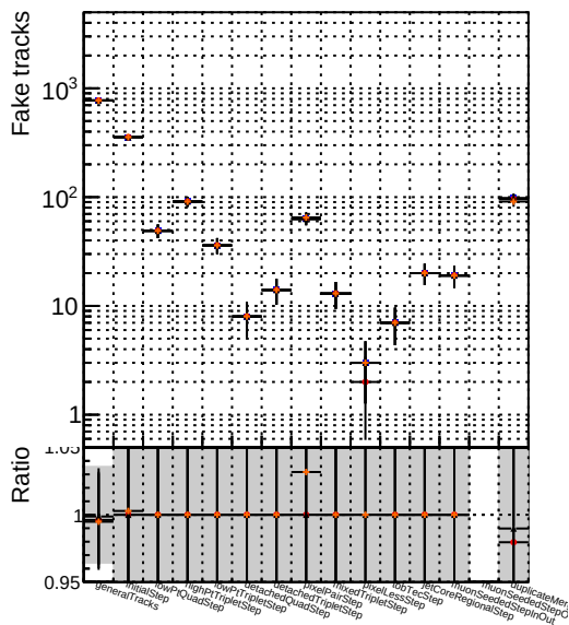
Number Color Model Order Scope Method Refinement 1 Red DOM V0001 R0000000001 Global mkFitNDOF RECO 2 Orange DOM V0001 R0000000001 Global mkFitNDOF2 RECO
