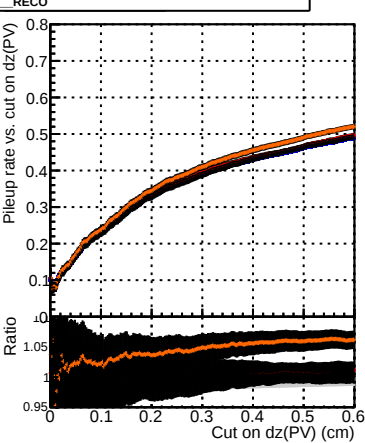
Pileup rate vs. cut on dz(PV)
