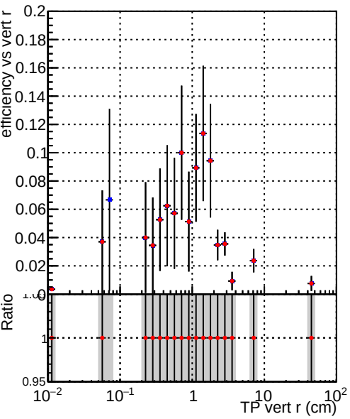
Efficiency vs vertpos Legend: DQM_V0001_R000000001_Global_CMSSW_100ti DQM_V0001_R000000001_Global_CMSSW_100timeHPTT
