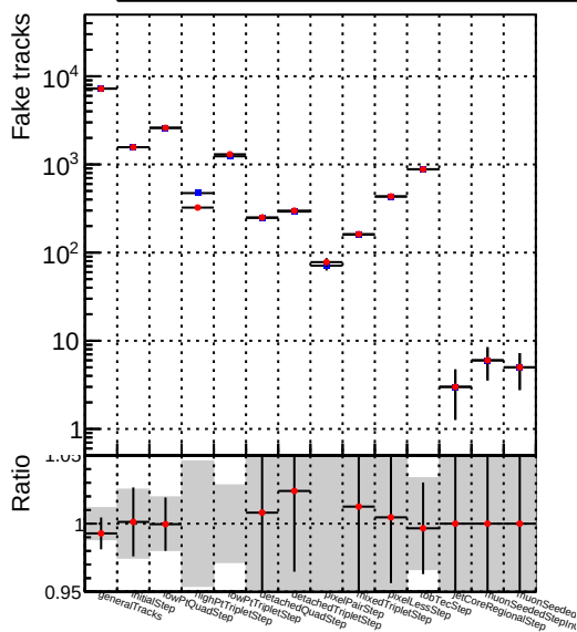
Number Label 1 DQM_V0001_R0000000001_Global_CMSSW_100timeHPTT
