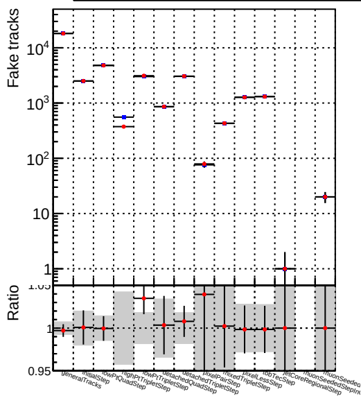
Number Legend DQM V0001 R0000000001 Global CMSSW 100timeHPTT
