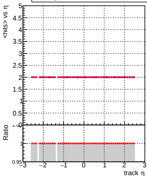
mean hits vs \eta Legend: DQM_V0001_R000000001_Global_CMSSW_100ti (blue line), DQM_V0001_R000000001_Global_CMSSW_100timeHPTT (red line)
