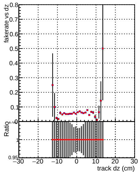
█ DQM_V0001_R0000000001 Global CMSSW_100ti █ DQM_V0001_R0000000001 Global CMSSW_100timeHPTT
