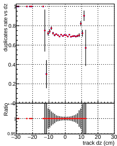
█ DQM_V0001_R0000000001 Global CMSSW_100ti █ DQM_V0001_R0000000001 Global CMSSW_100timeHPTT
