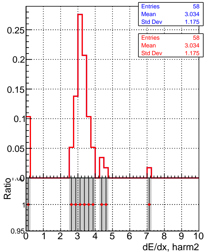
■ DQM_V0001_R000000001_Global_CMSSW_100ti ● DQM_V0001_R000000001_Global_CMSSW_100timeHPTT
