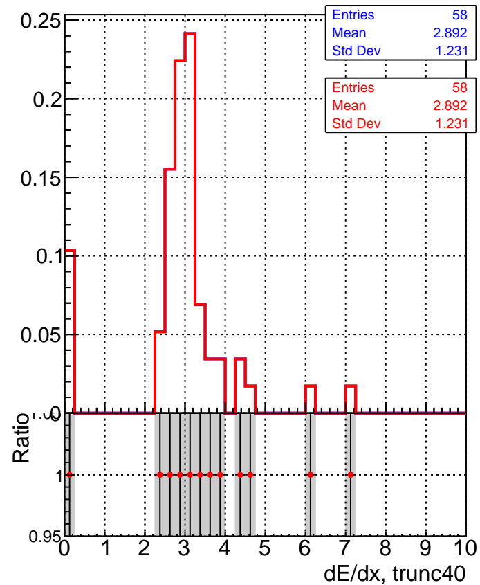
■ DQM_V0001_R000000001_Global_CMSSW_100ti ● DQM_V0001_R000000001_Global_CMSSW_100timeHPTT
