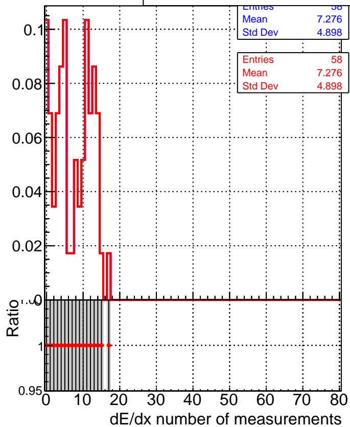
■ DQM_V0001_R000000001_Global_CMSSW_100ti ● DQM_V0001_R000000001_Global_CMSSW_100timeHPTT
