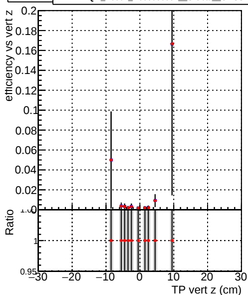
Efficiency — DQM_V0001_R0000000001_Global_CMSSW_100timeHPTT
