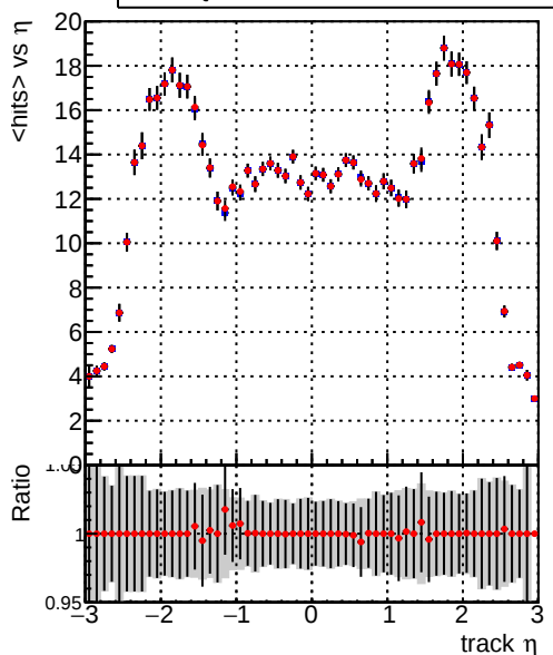
mean hit DQM_V0001_R000000001_Global_CMSSW_100ti DQM_V0001_R000000001_Global_CMSSW_100timeHPTT
