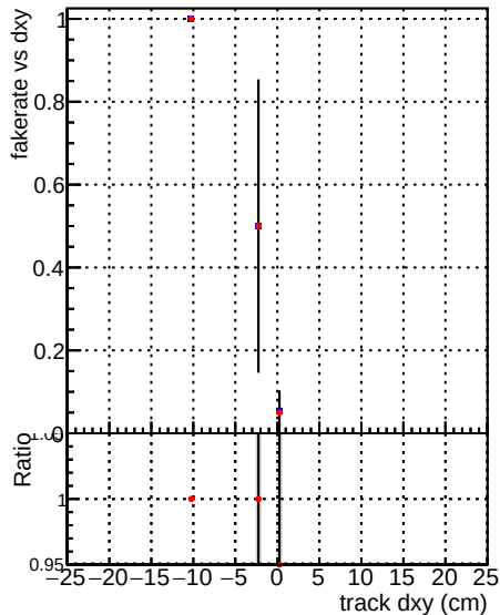
Legend Global CMSSW_100ti Fake rate vs d Blue dots and line DQM_V0001_R0000000001 DQM_V0001_R0000000001 Red dots and line DQM_V0001_R0000000001 DQM_V0001_R0000000001
