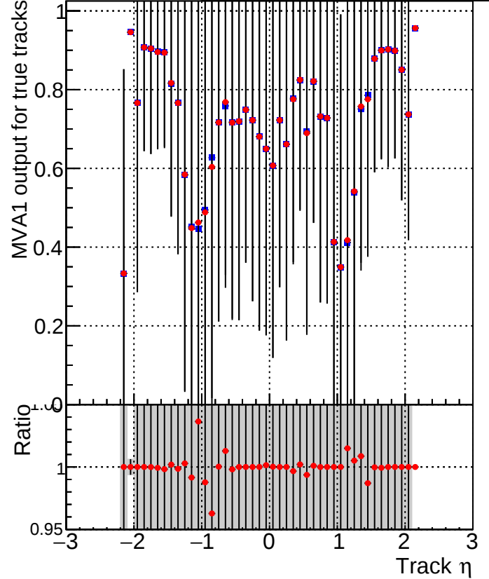
MVA1 of associated tracks (recoToSim) vs. track \eta Legend: ■ DQM_V0001_R000000001_Global_CMSSW_100ti ● DQM_V0001_R000000001_Global_CMSSW_100timeHPTT
