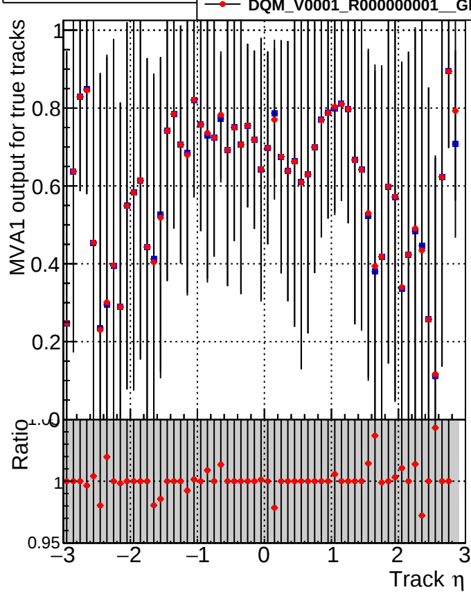
MVA1 of associated tracks (recoToSim) vs. track \eta
