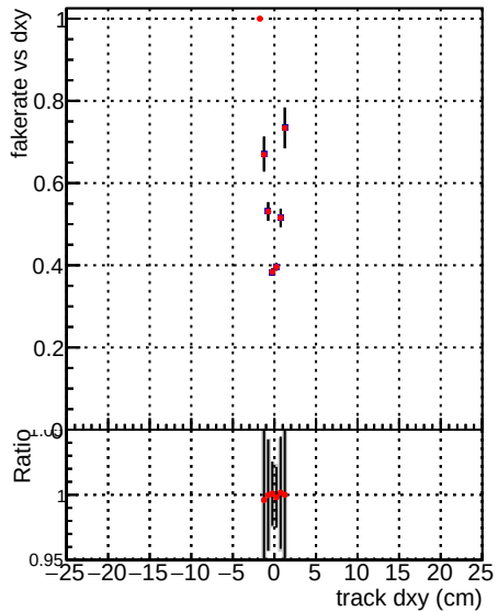
Global CMSSW_100ti Fake rate vs d DQM_V0001_R0000000001 DQM_V0001_R0000000001 Global CMSSW_100timeHPTT
