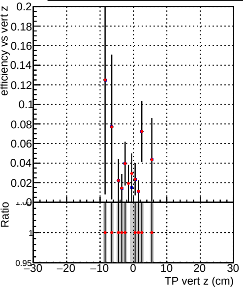
Efficiency vs vert z Legend: DQM_V0001_R000000001_Global_CMSSW_100ti DQM_V0001_R000000001_Global_CMSSW_100timeHPTT
