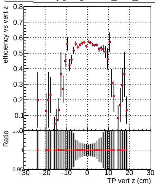
Efficiend —●— DQM_V0001_R0000000001_Global_CMSSW_100timeHPTT
