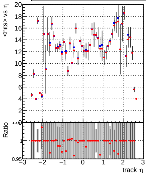
— DQM_V0001_R000000001_Global_CMSSW_100ti — DQM_V0001_R000000001_Global_CMSSW_100timeHPTT
