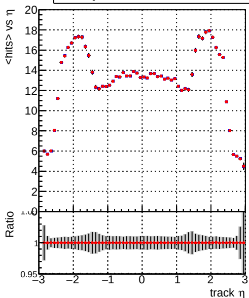
mean hits vs \eta — DQM_V0001_R000000001_Global_CMSSW_100ti — DQM_V0001_R000000001_Global_CMSSW_100timeHPTT
