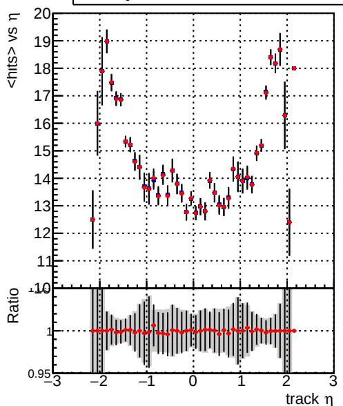
— DQM_V0001_R000000001_Global_CMSSW_100ti — DQM_V0001_R000000001_Global_CMSSW_100timeHPTT
