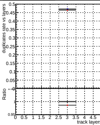
Duplicates Rate vs layer
