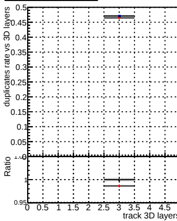
Duplicates Rate vs 3D layer
