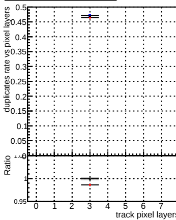
Duplicates Rate vs pixel layer
