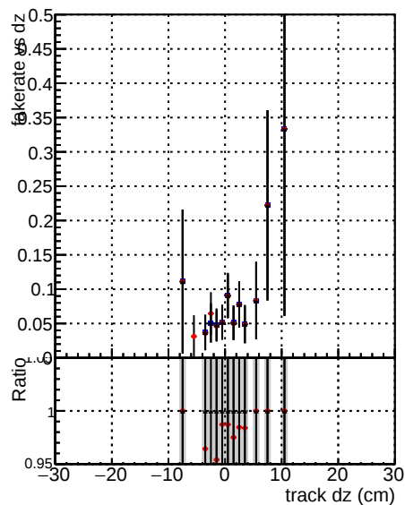
DOM V0001 R0000000001 Global CMSSW_100ti DOM V0001 R0000000001 Global CMSSW_100ti DOM V0001 R0000000001 Global CMSSW_100ti
