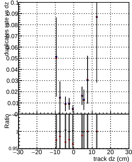
CMSSW-100timeHPIT CMSSW-100timePLa
