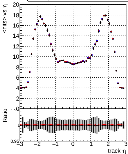
mean hits vs \eta Legend: DQM_V0001_R000000001_Global_CMSSW_100ti DQM_V0001_R000000001_Global_CMSSW_100timeHPTT DQM_V0001_R000000001_Global_CMSSW_100timePLa
