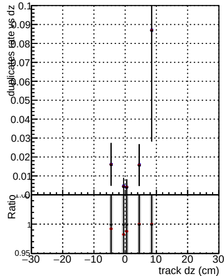
CMSSW_100timeHPIT CMSSW_100timePLa
