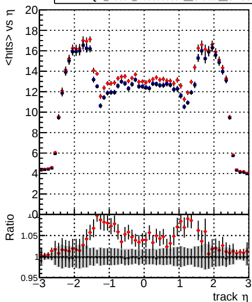
mean hits vs \eta Legend: DQM_V0001_R000000001_Global_CMSSW_100ti (blue line), DQM_V0001_R000000001_Global_CMSSW_100timeHPTT (red line), DQM_V0001_R000000001_Global_CMSSW_100timePLa (black line)
