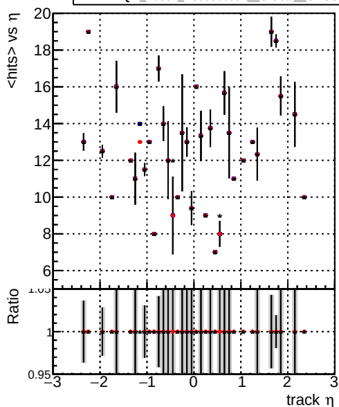
mean hits DQM_V0001_R000000001_Global_CMSSW_100ti DQM_V0001_R000000001_Global_CMSSW_100timeHPTT DQM_V0001_R000000001_Global_CMSSW_100timePLa
